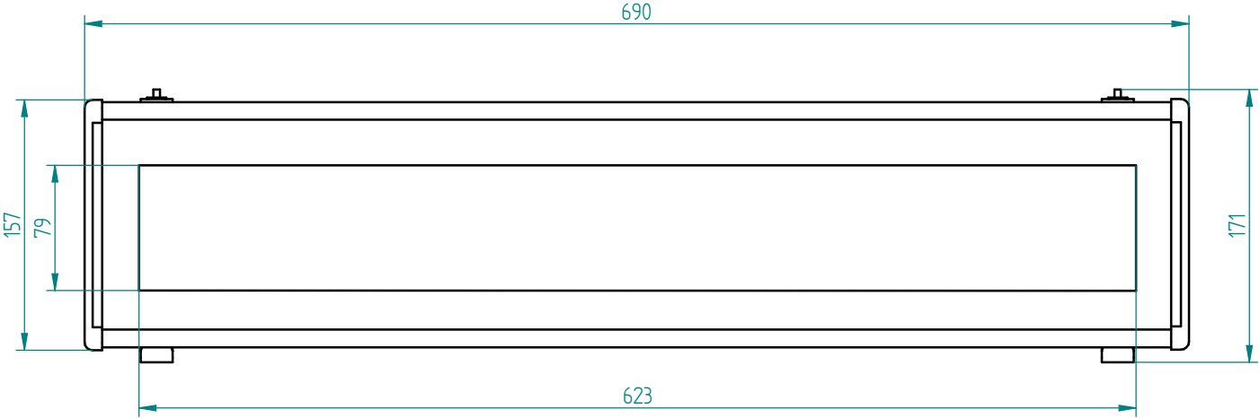
Vista frontal
