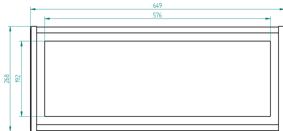
Vista frontal
