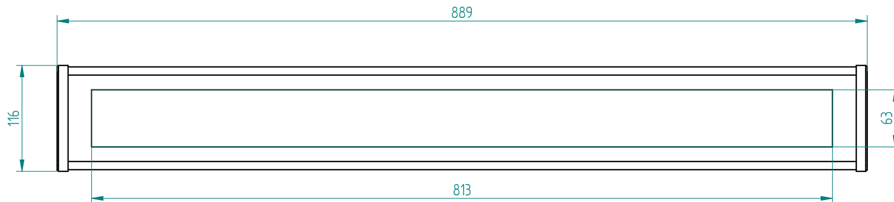
Vista frontal
