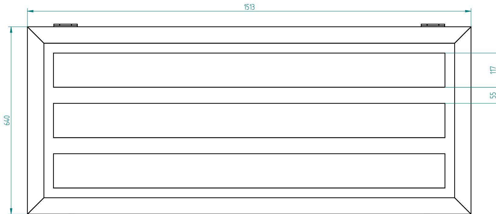
Vista frontal
