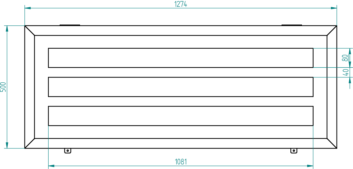
Vista frontal
