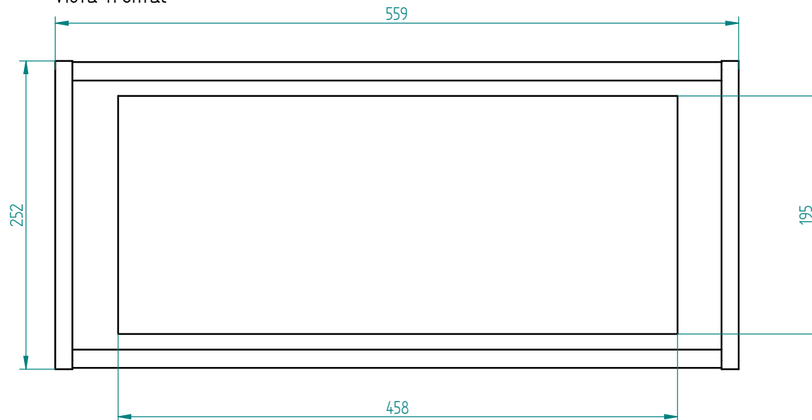
Vista frontal
