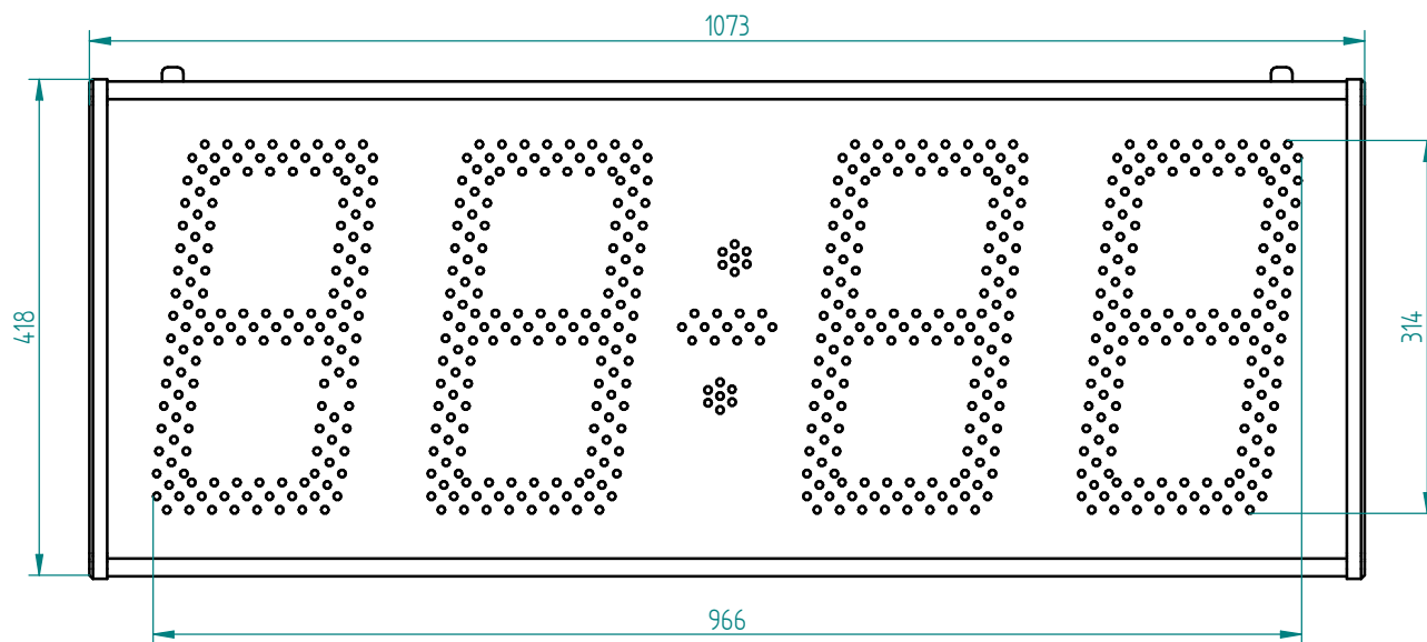
Vista frontal
